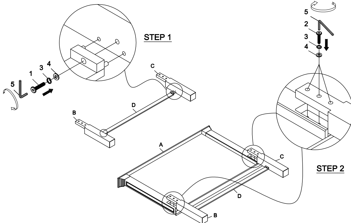
Complete Assembly
