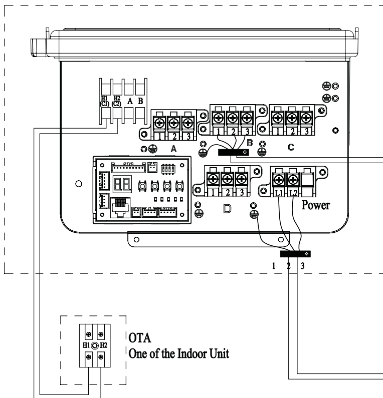
Outdoor unit
