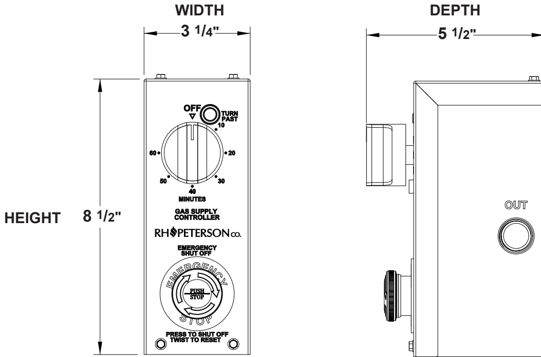
Fig. 2-1 Commercial dimensions
