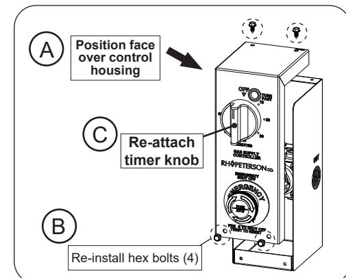
Fig. 4-4 Reinstall control face
