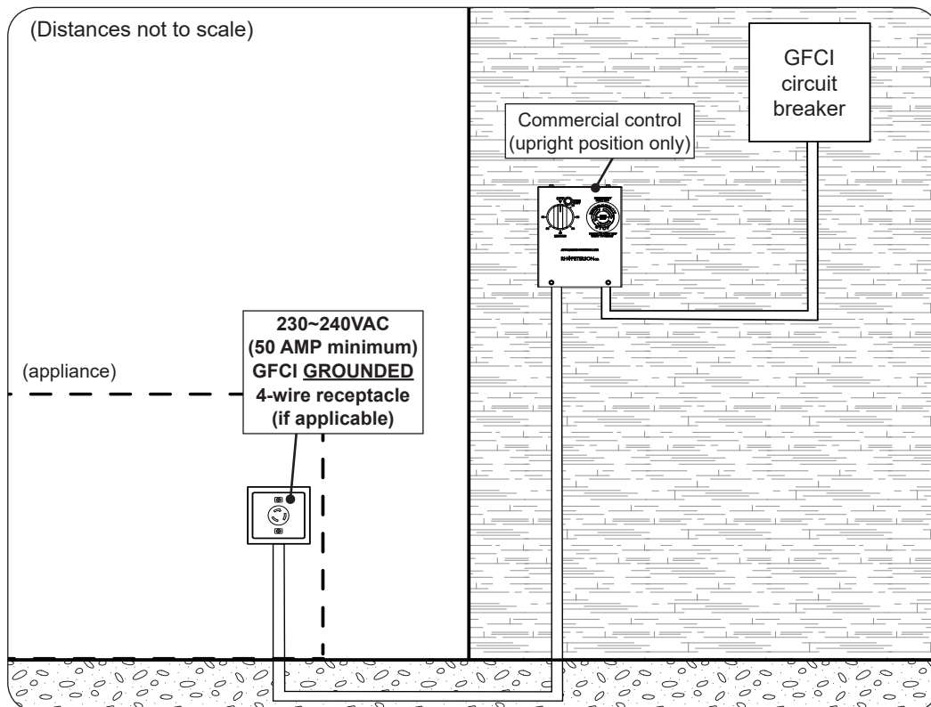
Fig. 2-2 Installation overview
