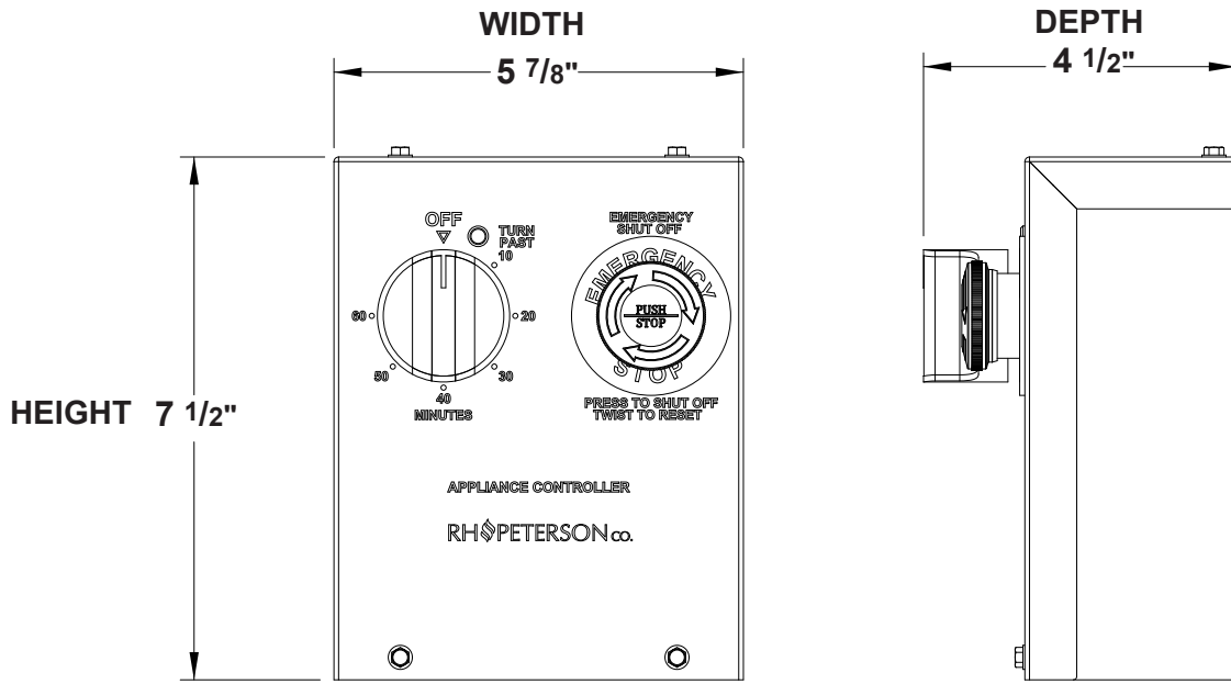
Fig. 2-1 Commercial dimensions
