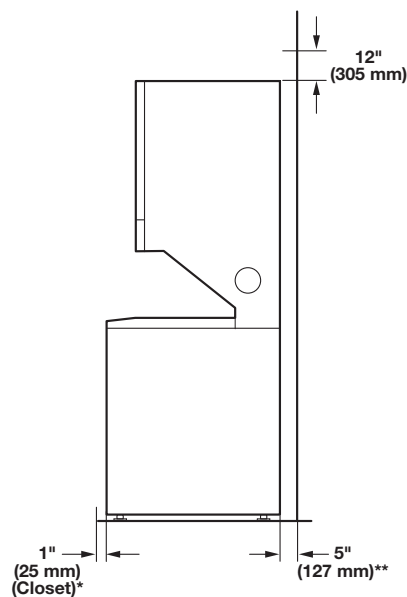
Front/Back/Top Clearances
