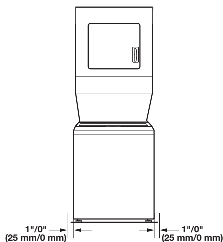
Side Clearances (recommended/minimum)
