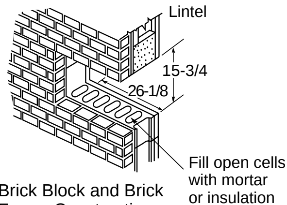
Frame Construction
