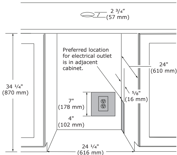
Cabinet Cut-Out
