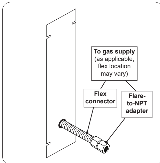
Fig. 26-1 Connect gas and secure plate
