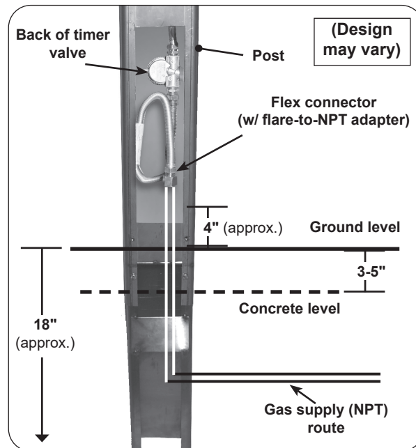
Fig. 27-1 In-ground install orientation
