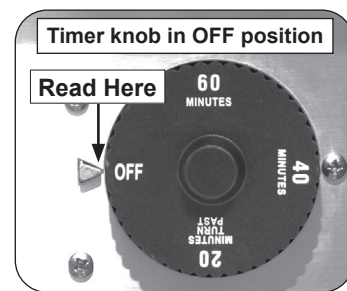
Fig. 35-3 Timer dial
