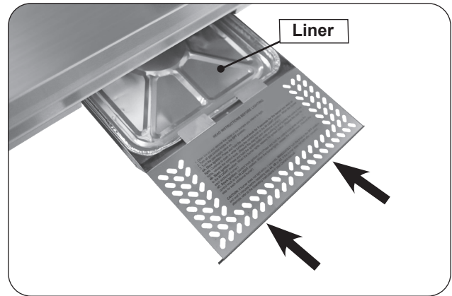
Fig. 32-1 Install drip tray
