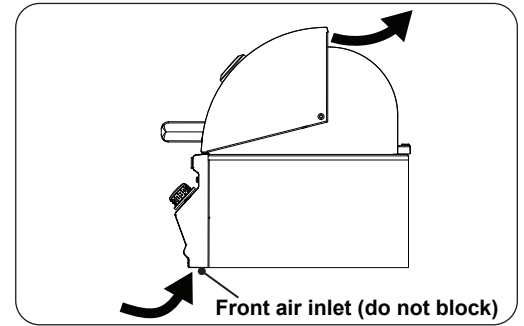
Fig. 16-1 Airflow diagram
