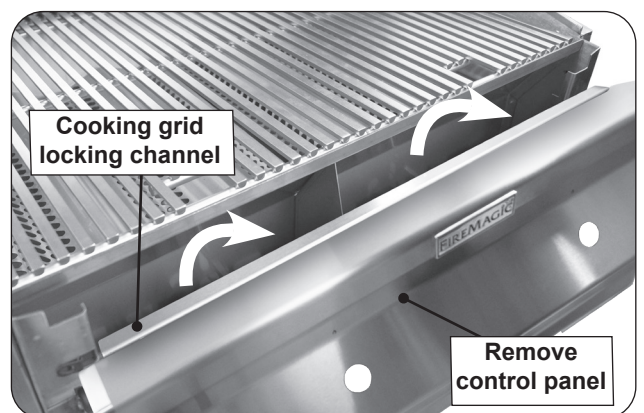
Fig. 39-4 Control panel removal
