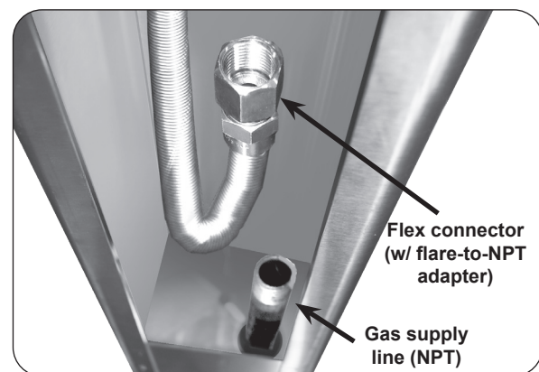
Fig. 27-2 Post interior detail
