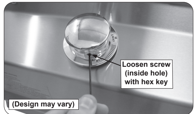
Fig. 39-2 Loosen screw to free knob
