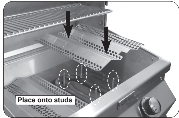
Fig. 30-1 Install flavor grids
