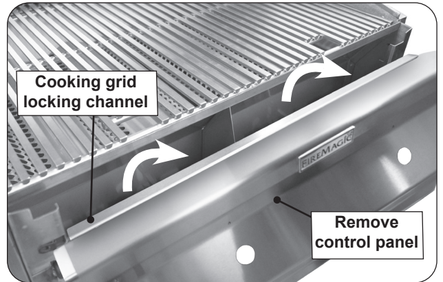
Fig. 40-1 Control panel / grid locking channel removal
