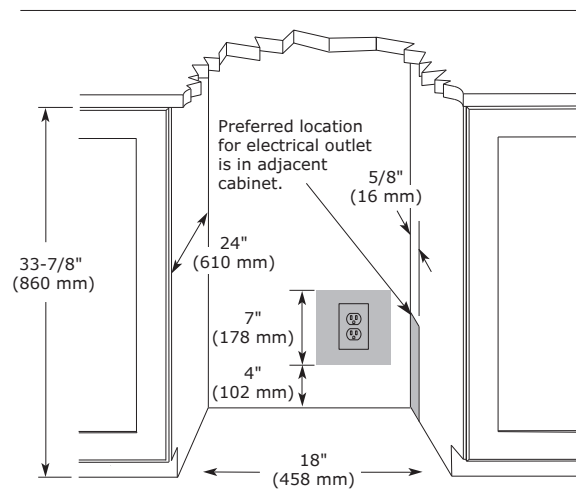
Cabinet Cut-Out
