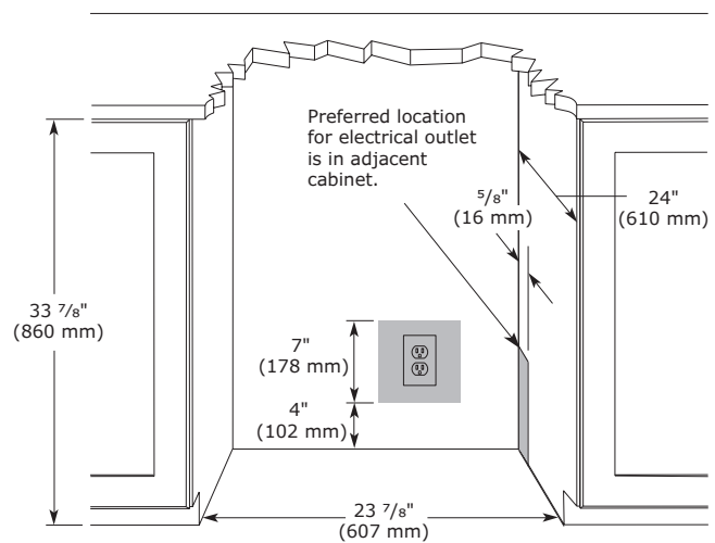
Cabinet Cut-Out
