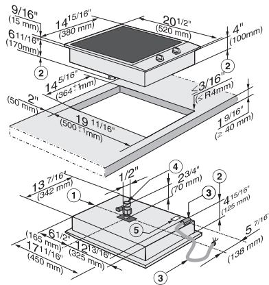
CS 1322 BG (installation drawing) – USA
