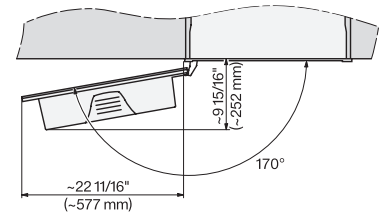
CVA7440, CVA7445, CVA7840, CVA7845, installation drawing, view from above, 60 cm, Proud
