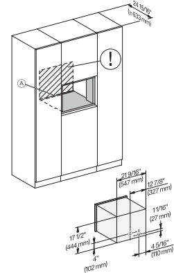
CVA7445, CVA7845, installation drawing, 60 cm, Flush inset
