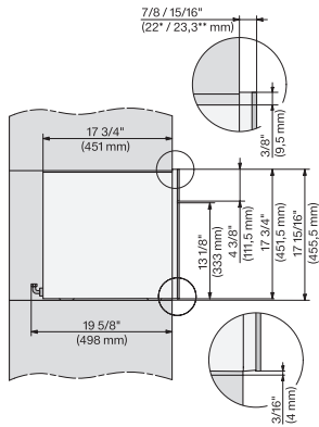
CVA7445, CVA7845, side view, 60 cm, Proud 7/8" – 22* mm – Glass, 15/16" – 23.3** mm – Stainless steel
