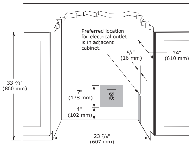
Cabinet Cut-Out
