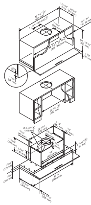
DA 3698, DA 3698 EXT (Installation drawing) – US
