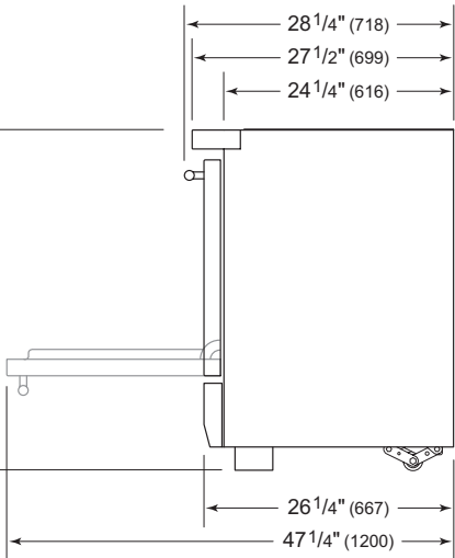
SIDE VIEW—TRANSITIONAL
