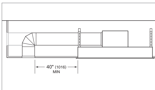
Recirculating application
