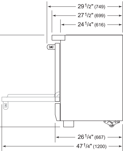
SIDE VIEW—PROFESSIONAL
