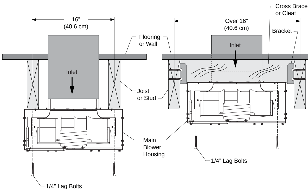
Mounting on Joists or Studs Spaced 16"
