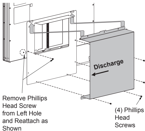
Discharge Left
