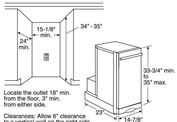
Compactor Dimensions (in inches)
