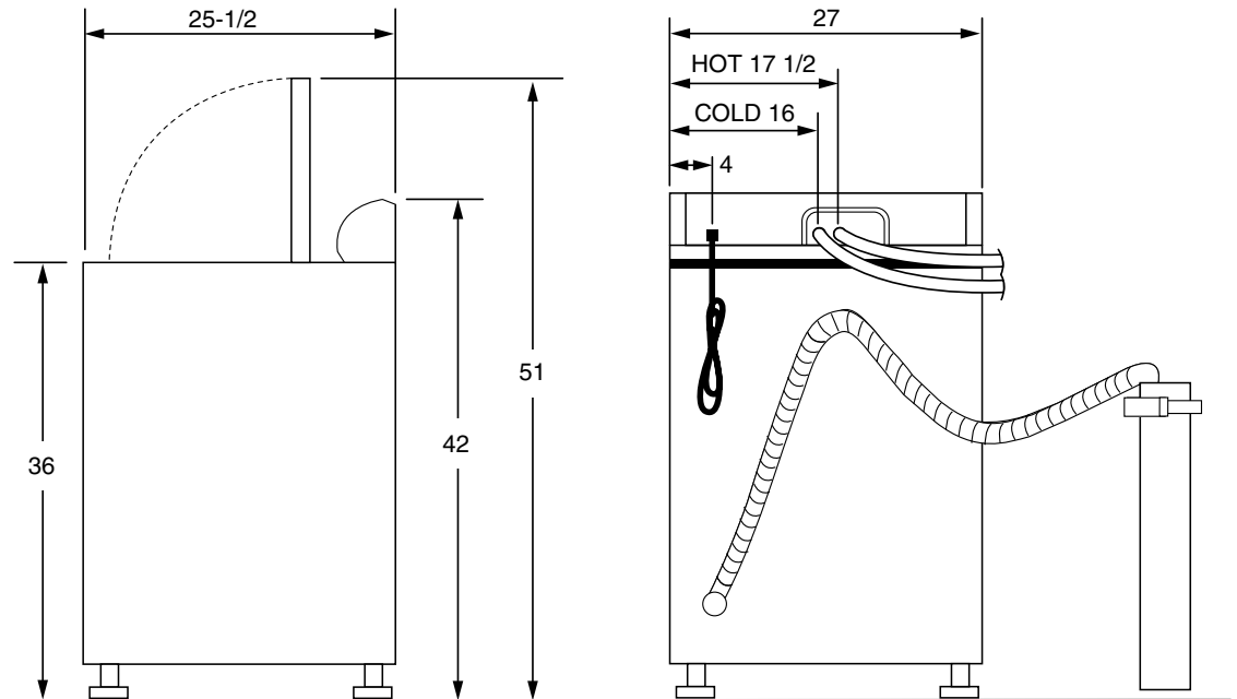
Side View
