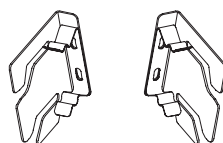
Fully Integrated Grille Bracket W10260890—Left (1) W10260891—Right (1)
