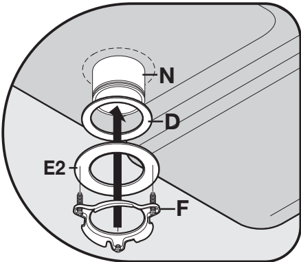
FIGURE C: Extra Thick Sink For Model KBDS100T Only ( > 3/4" )
