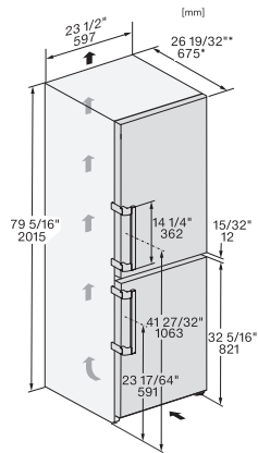
KFN4799DDE, installation sketch (US)
