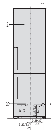
KFN4799DDE, installation (US)
