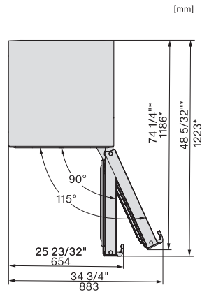
KFN4799DDE, top view (US)
