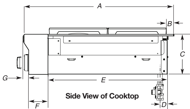
A. 27 \frac{3}{4} " (70.5 cm) B. 1 \frac{1}{4} " (3.2 cm) C. 7 \frac{7}{16} " (18.8 cm) D. Gas inlet is located 1 \frac{7}{8} " (4.8 cm) from the back of the cooktop burner base and 4 \frac{7}{8} " (12.4 cm) in from left-hand side of the cooktop burner base.
