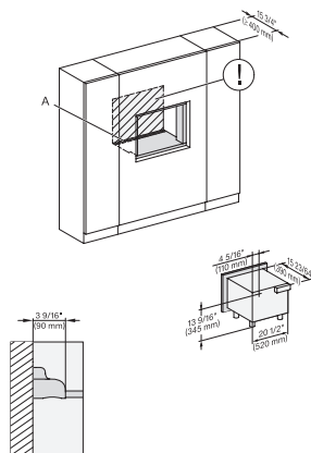
M2241SC, Installation, 30 Zoll, Flush, inset, breite Front – Skizze – NA
