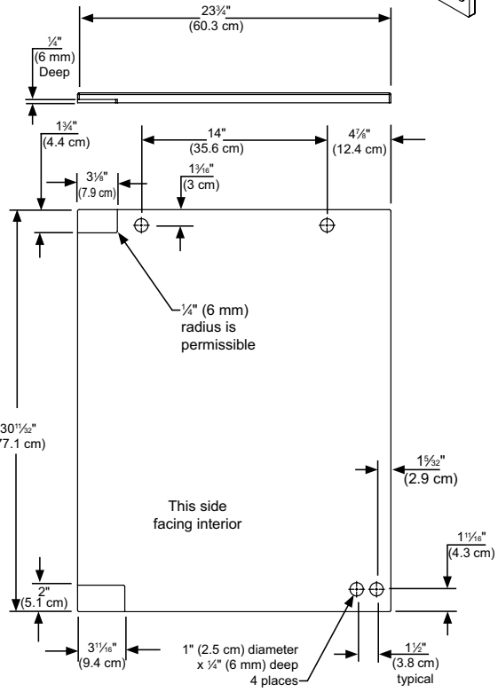
Right Hand Hinged Door 24" (61 cm) wide appliance
