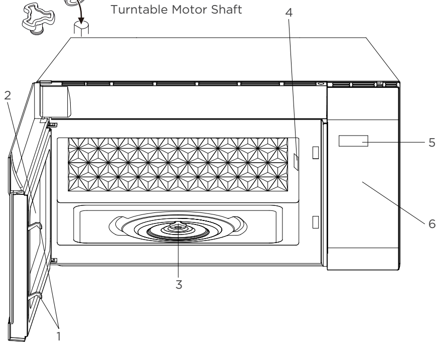
Turntable Motor Shaft
