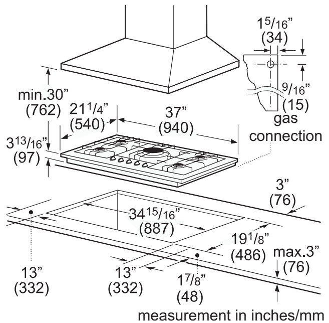
Figure 2: Cutout Dimensions
