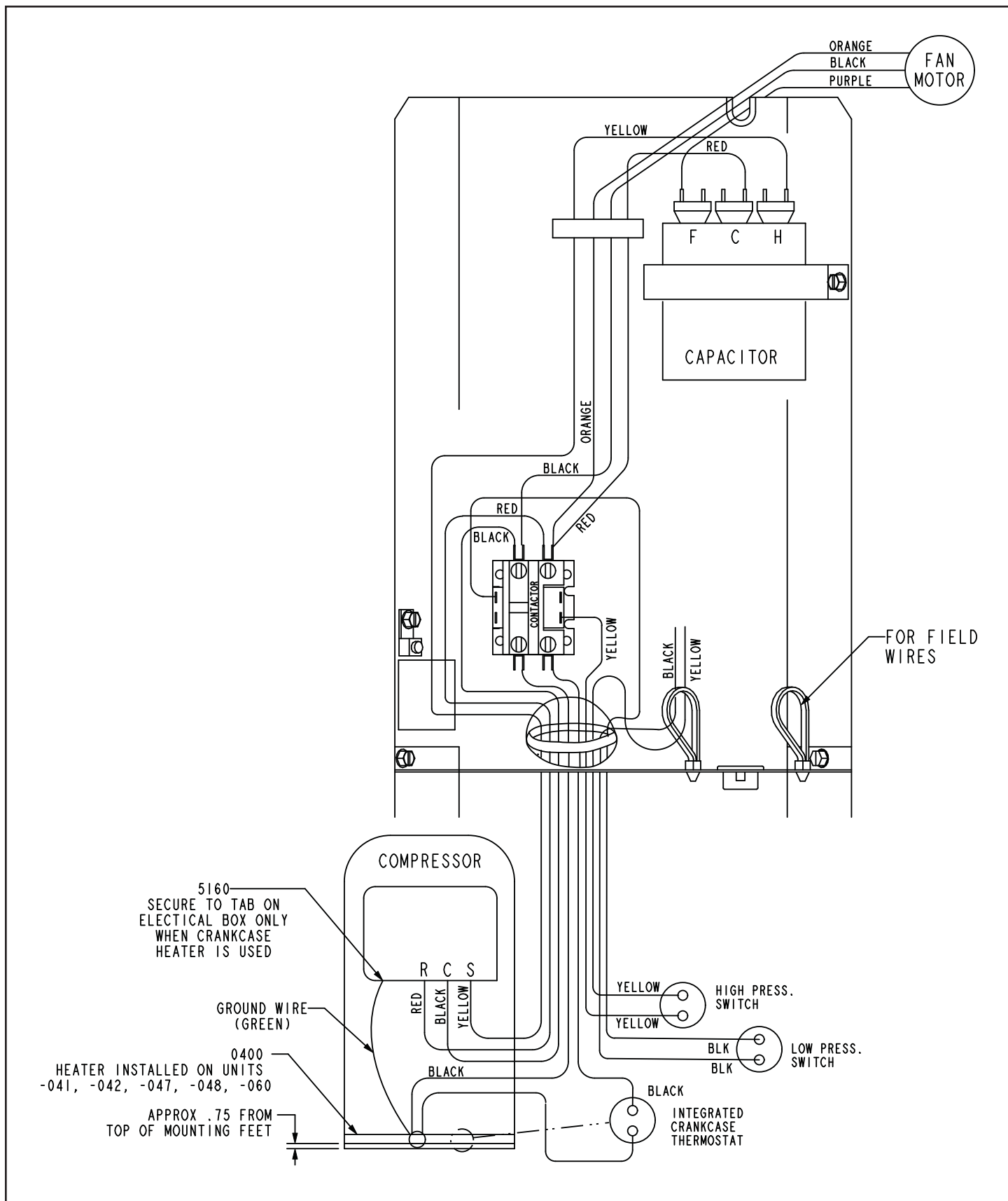
FIGURE 16. Typical Factory Wiring Diagram – -018, -024, -030, -036, -048, and -060 Units Only
