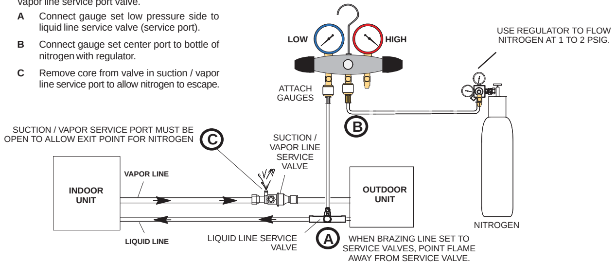
FIGURE 8. Brazing Procedures
