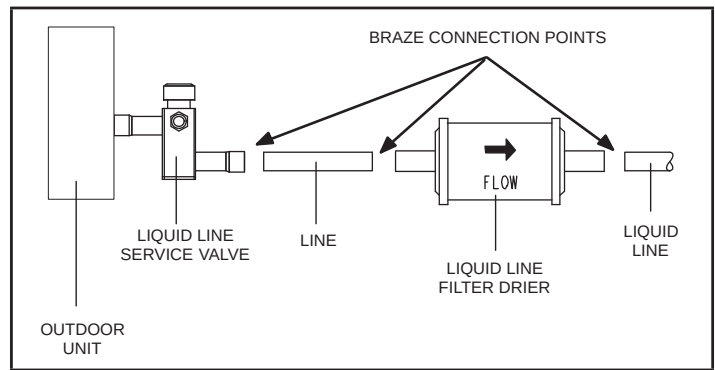
FIGURE 6. Typical Liquid Line Filter Drier Installation
