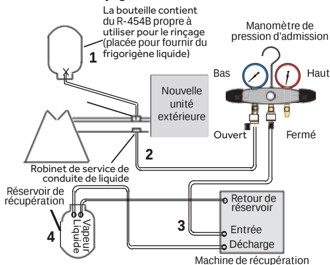
Figure 15. Raccordement des jauges
