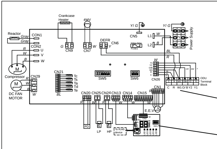
Figure 19. 18K/24K/30K/36K/42K/48K Wiring Diagram
