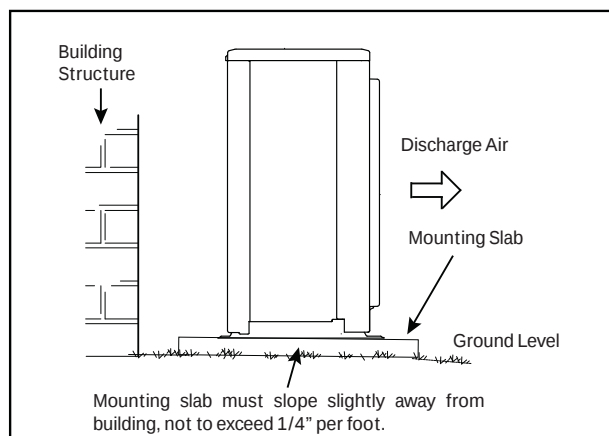
Figure 1. Slab Mounting
