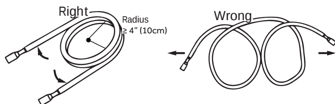
Figure 4. Minimum Bend Radius
