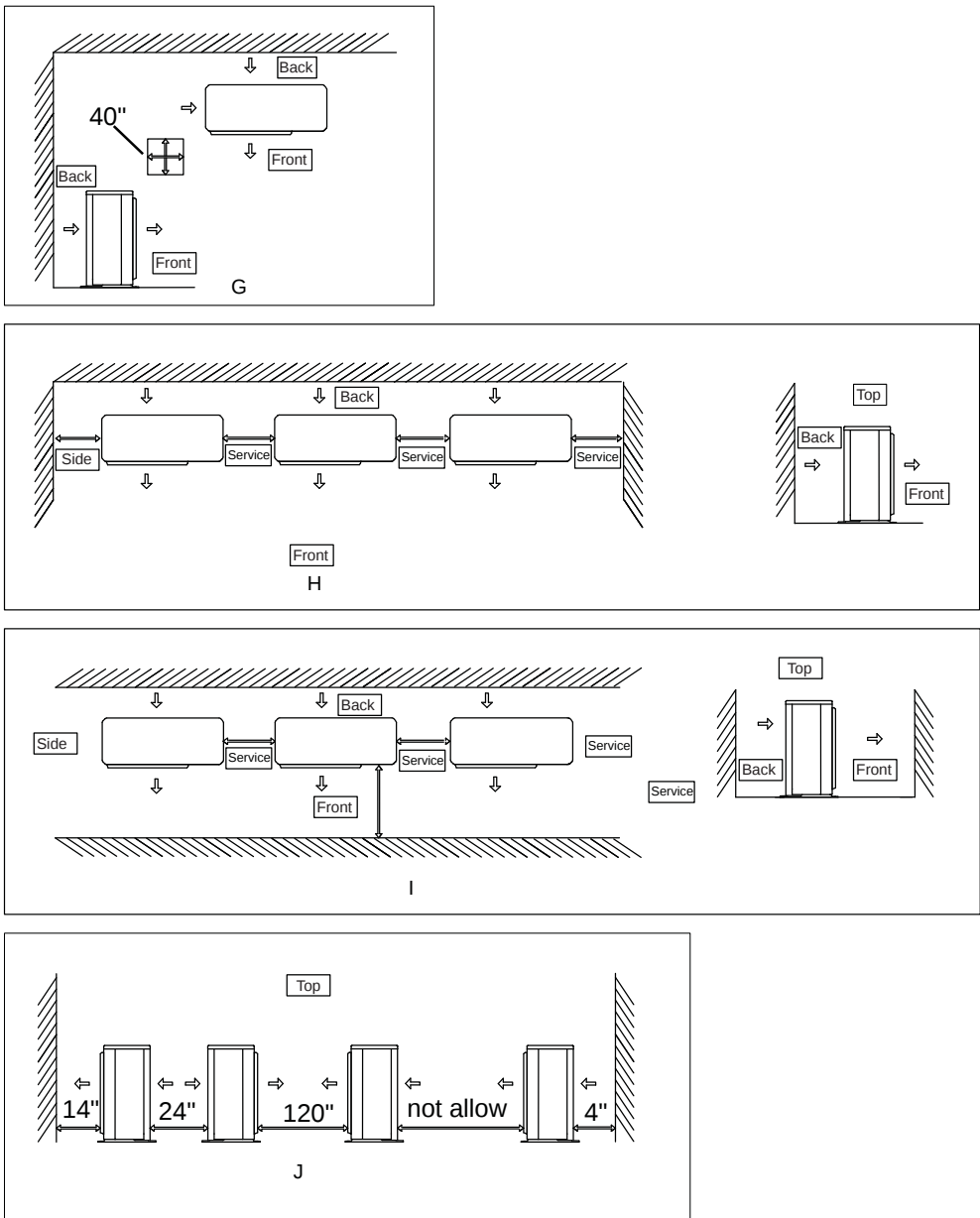
Figure 3. Multiple-Unit Clearance Configuration
