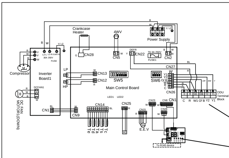
Figure 20. 60K Wiring Diagram
