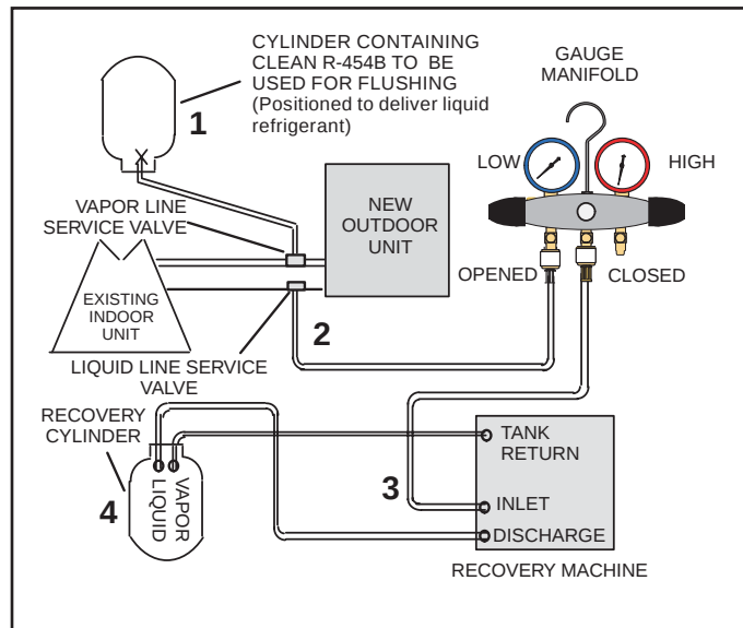
Figure 15. Connecting Gauges
