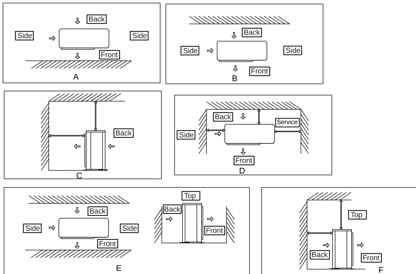
Figure 2. Single-Unit Clearance Configurations
