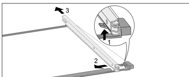
Fig. 131 Glass shelf with rails
