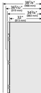
RIGHT VIEW
