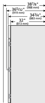
RIGHT VIEW
