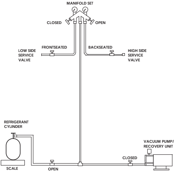
CHARGING CONNECTIONS
