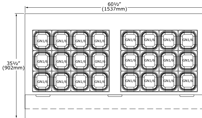
Drawer Interior (UCMT160-SS91A)
