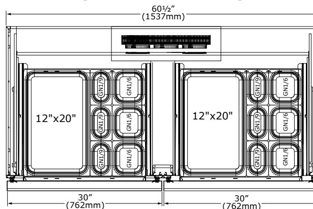
Drawer Interior (UCMT160-SS91A)
