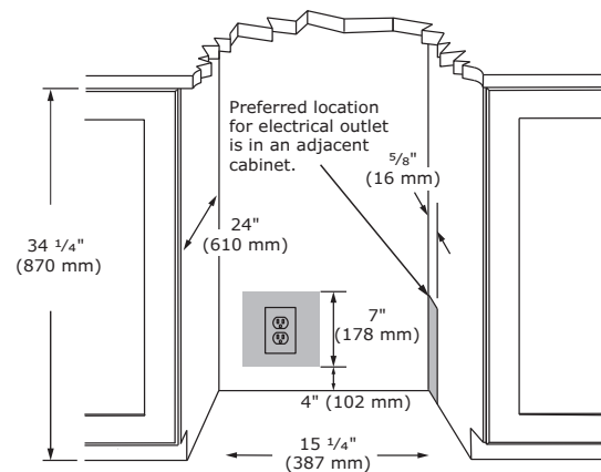
Cabinet Cut-Out
