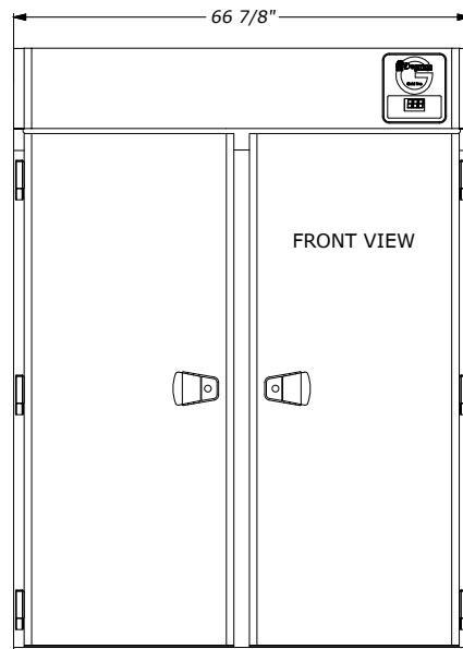
Front UCRE666 (Open)
