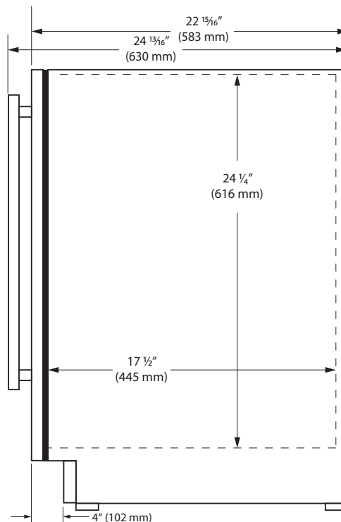
Cabinet Cut-Out
