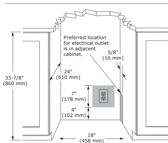
Cabinet Cut-Out
