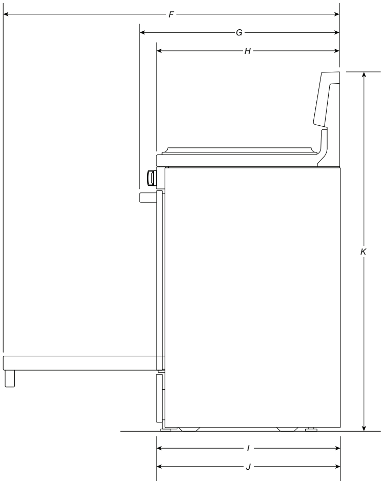
SIDE VIEW
