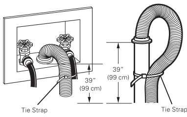
Tie Strap
