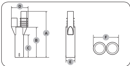
Dimensions of the pipe connector
